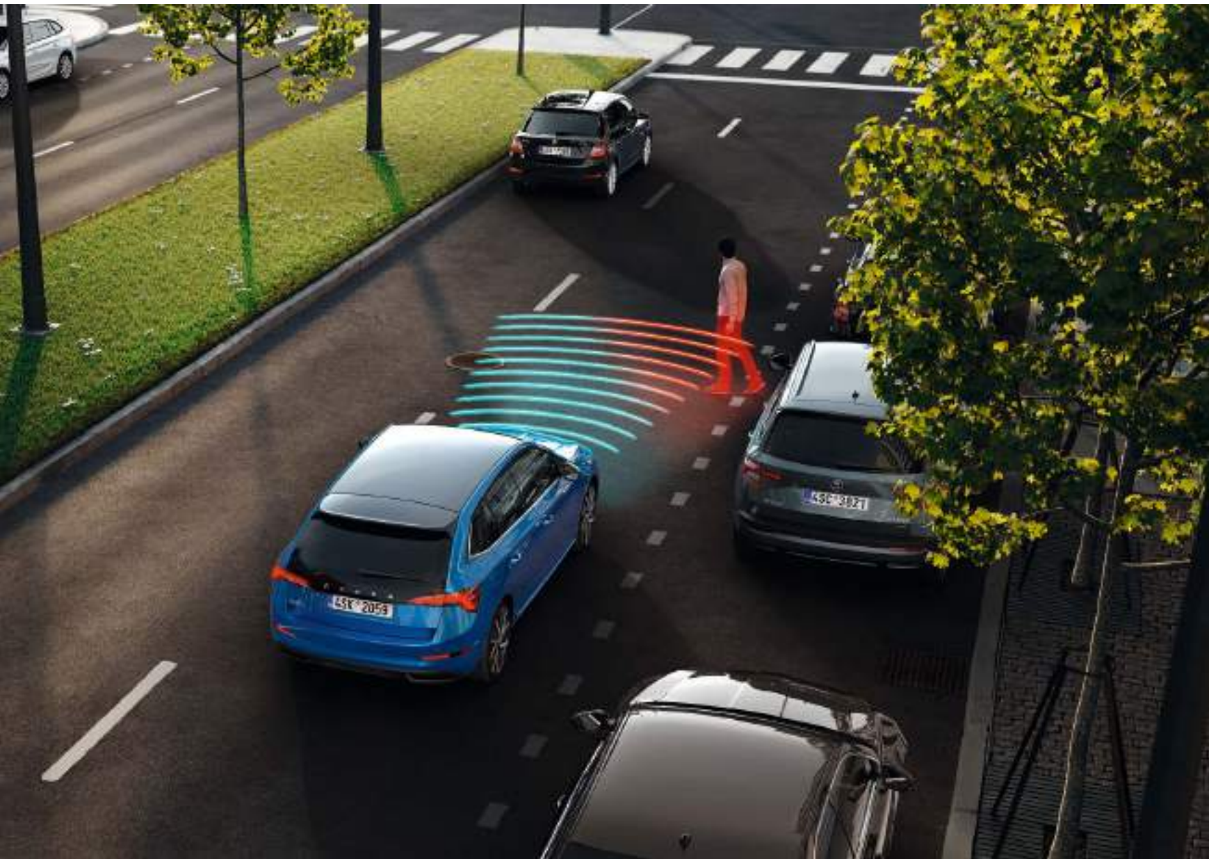
FRONT ASSIST WITH PREDICTIVE PEDESTRIAN PROTECTION The Front Assist system, using a radar device in the front grille, is designed to monitor the distance from the vehicle ahead, including emergency braking function. The SCALA comes with Front Assist expanded with predictive pedestrian protection, which warns the driver via an audio/visual signal as well as a gentle jolt of the brakes.
